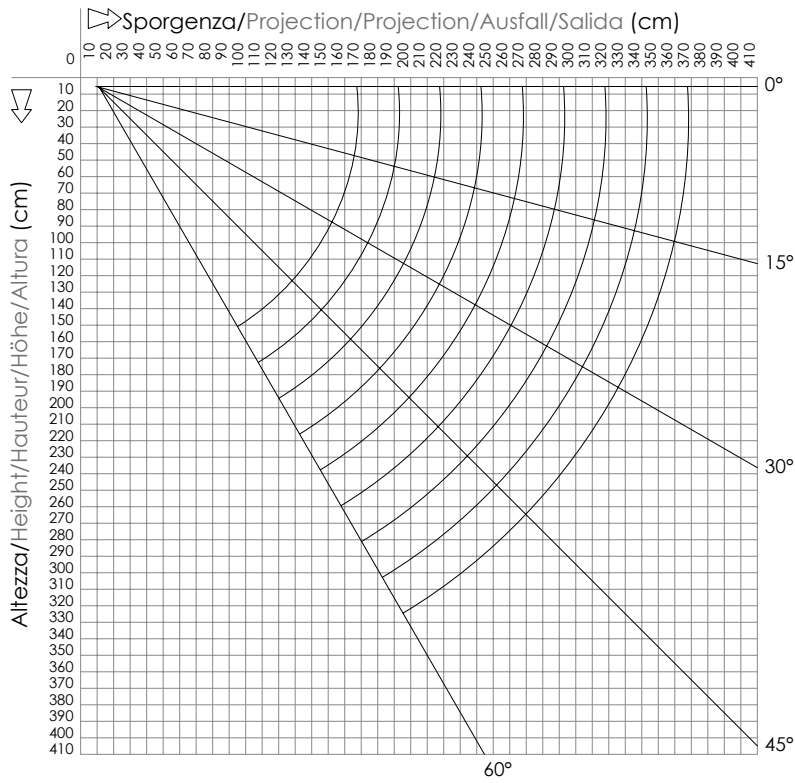
Montaggio a parete Wall installation
