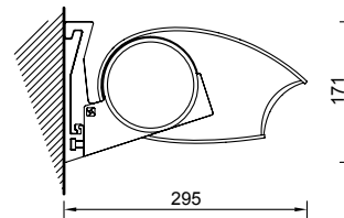
Montaggio a parete Wall installation
